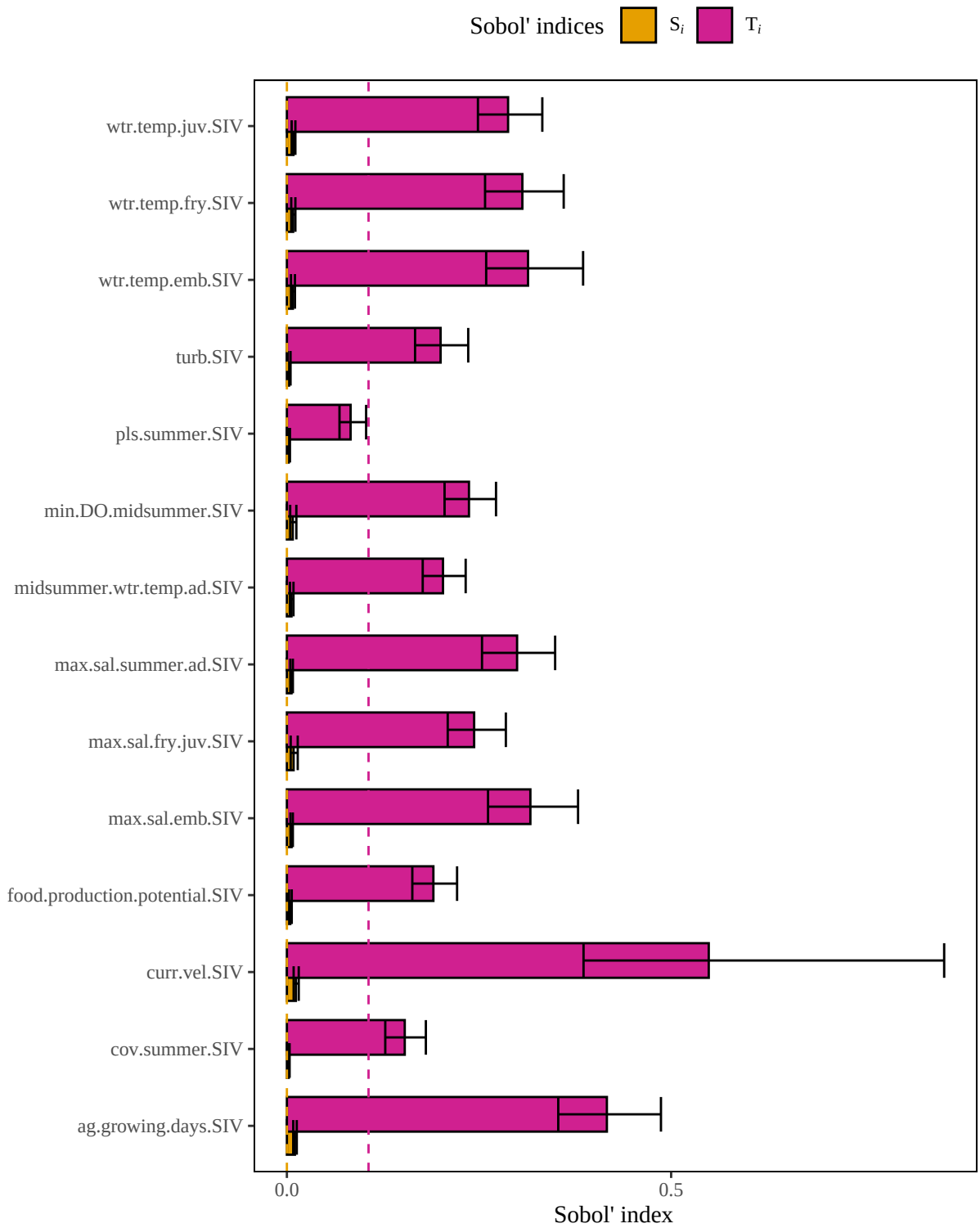
Figure 7. Results of a sensitivity analysis for the channelcatfishRiv model based on a multiplicative mean structure. Dashed lines represent baseline numerical approximation error for S_i and T_i ( i.e. , dummy variables).
